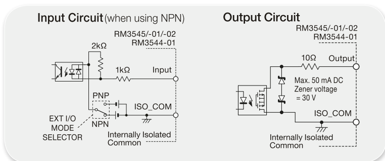
EXT I/O polarity (Select NPN/PNP)
