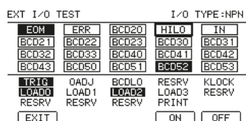
EXT I/O test function screen
