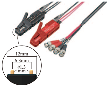
CLIP TYPE PROBE L2002 Cable length 1.5 m (4.92 ft)
